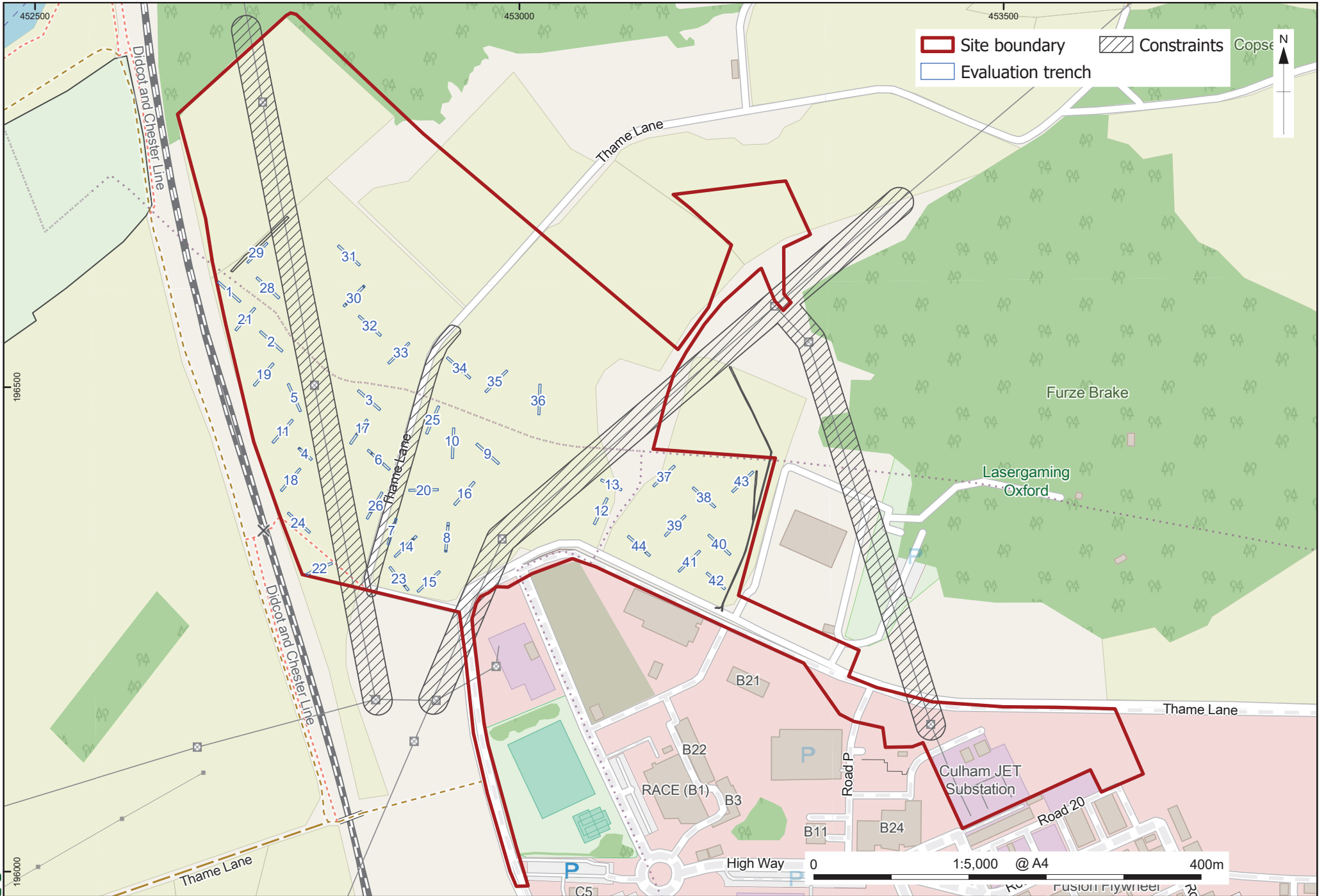
Figure 2: Location of evaluation trenches
