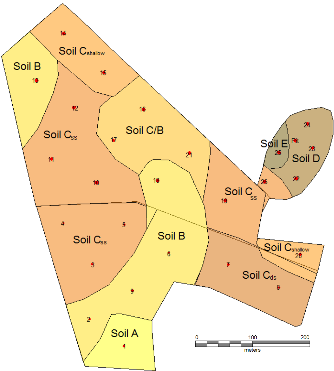
Map 3: Soil type map for the Culham site
